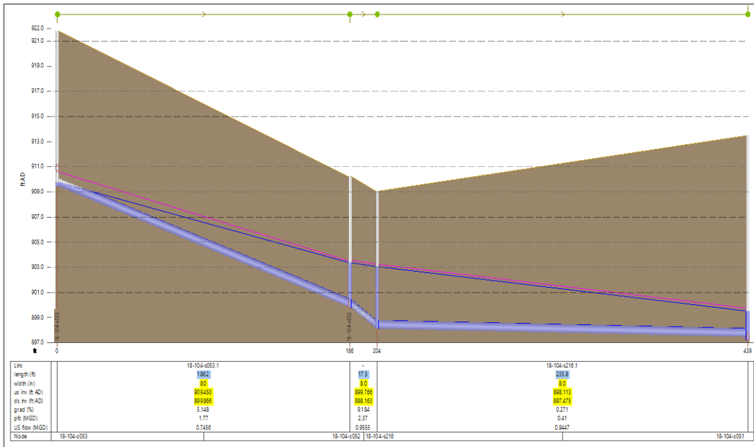
Hydraulic profile of 2 year design storm
