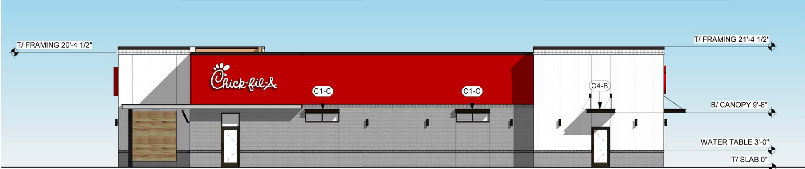
EXTERIOR ELEVATION 1" = 10'-0"
