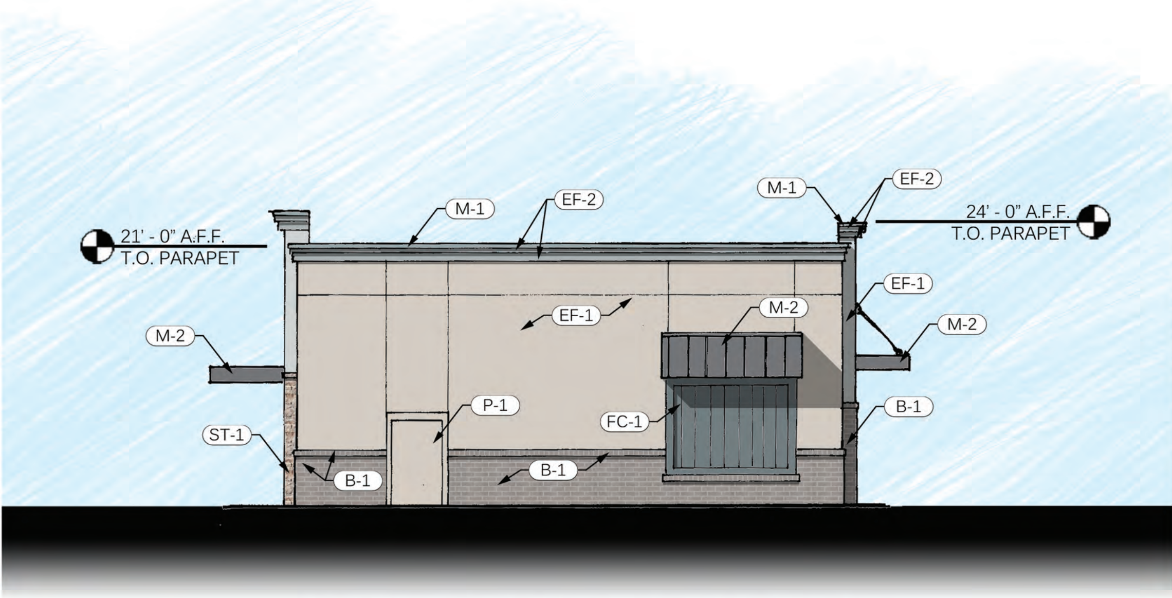
REAR ELEVATION
