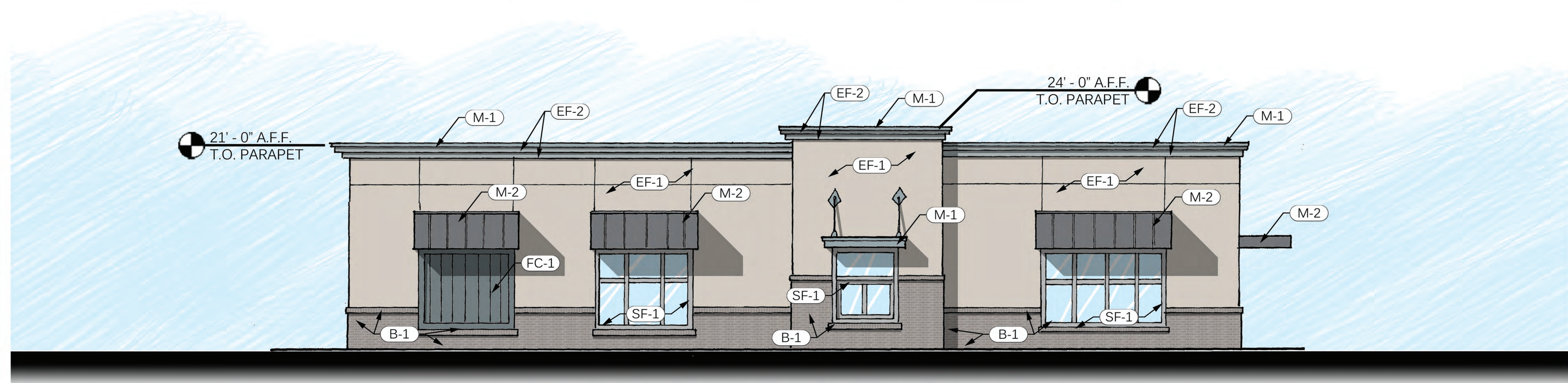
DRIVE-THRU ELEVATION
