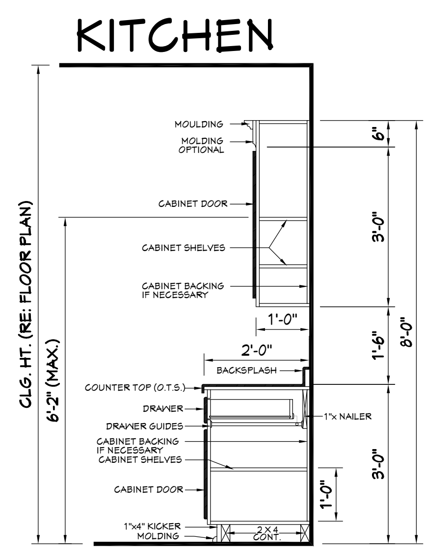
606 TYPICAL CABINET SECTIONS SCALE-----N.T.S.
