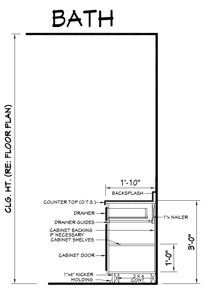
606 TYPICAL CABINET SECTIONS SCALE-----N.T.S.
