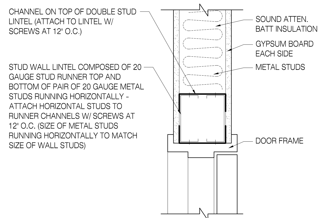
1 Door Head Detail 3" = 1'-0"
