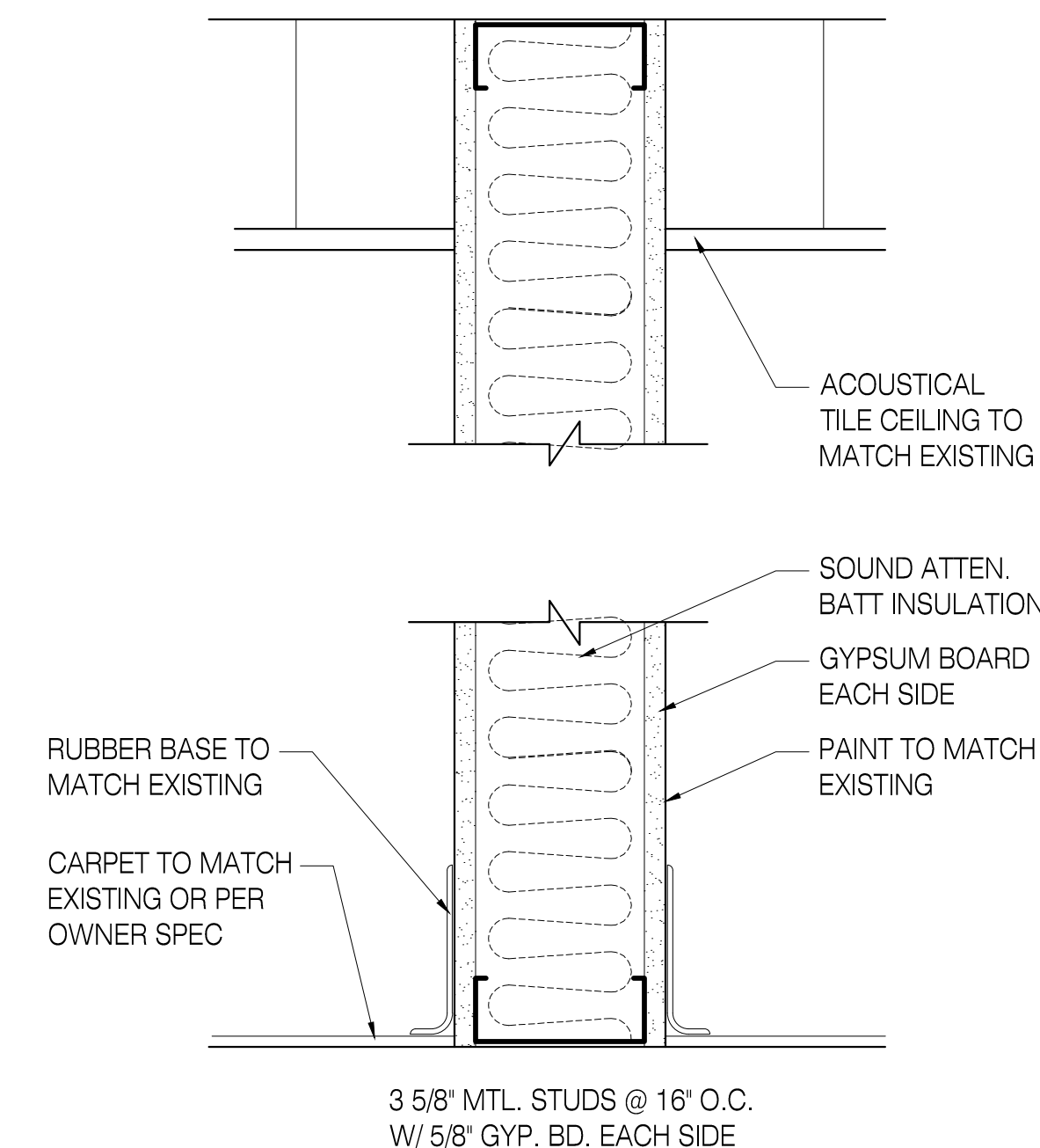
4 Typ. Wall Section 3" = 1'-0"
