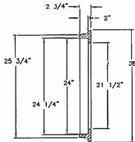
FRAME SECTION
