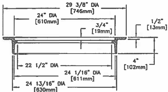
FRAME SECTION
