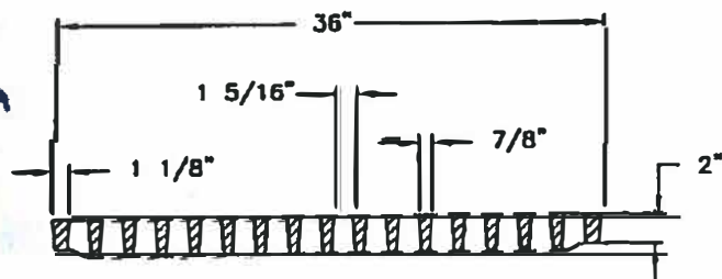
GRATE SECTION
