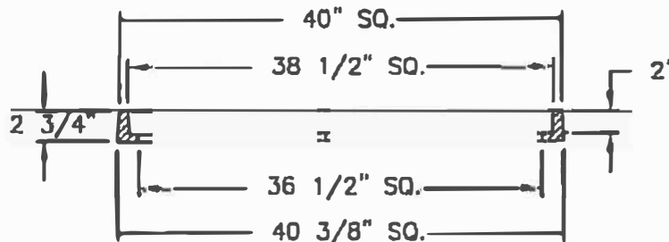
FRAME SECTION
