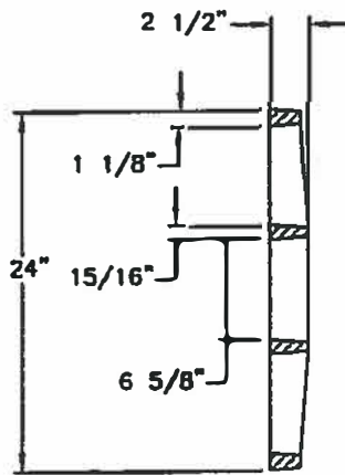
GRATE SECTION
