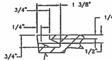
PICKHOLE DETAIL
