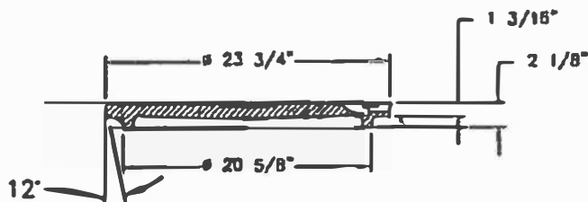
COVER SECTION
