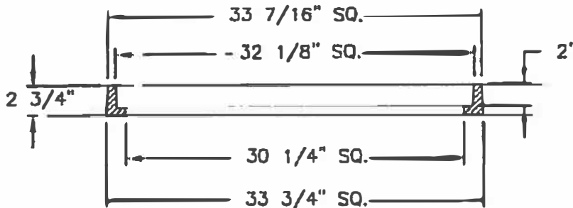
FRAME SECTION
