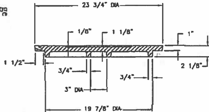
COVER SECTION
