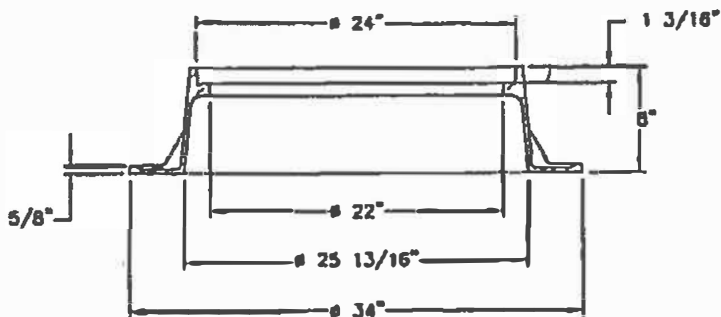
FRAME SECTION
