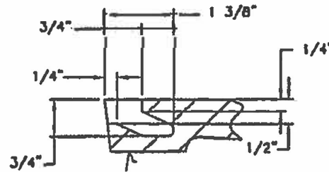
PICKHOLE DETAIL
