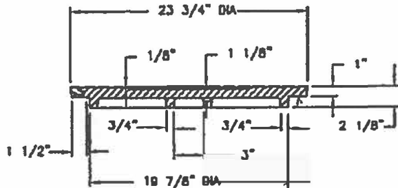
SECTION OF COVER
