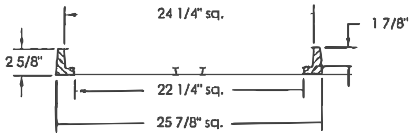
FRAME SECTION
