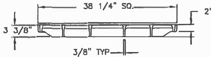
GRATE SECTION
