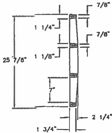
GRATE SECTION
