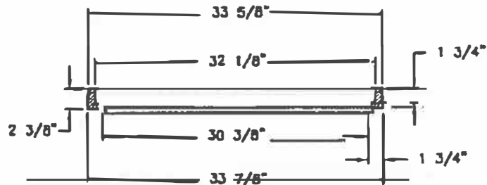
FRAME SECTION
