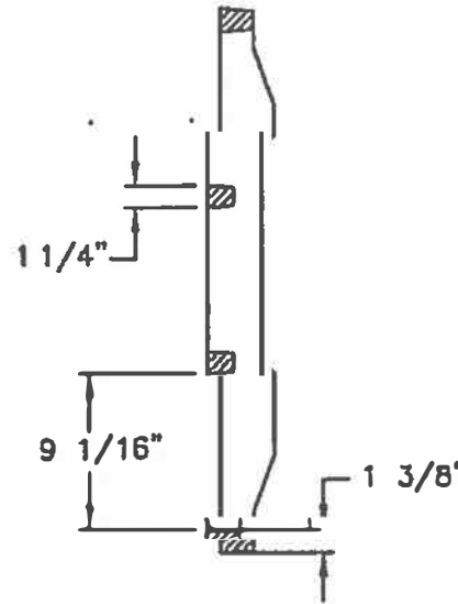
GRATE SECTION
