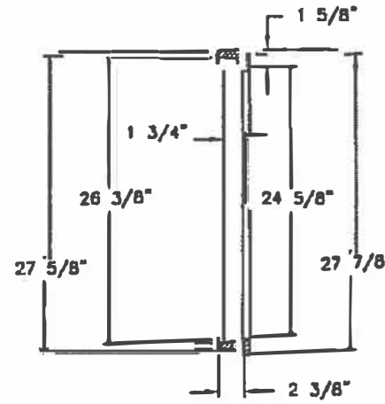
FRAME SECTION
