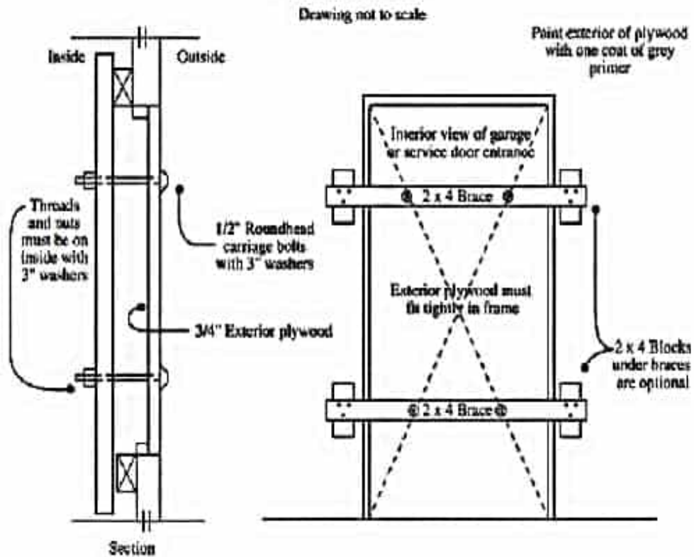
Drawing 1 – Boarding up doors
