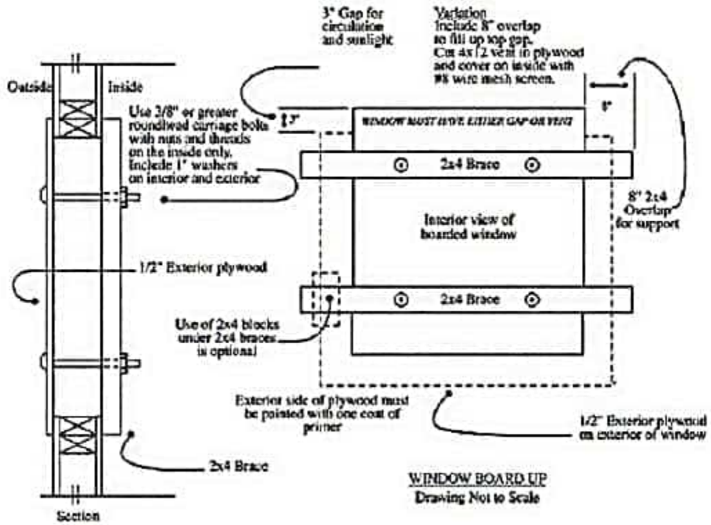
Drawing 2 – Boarding up windows
