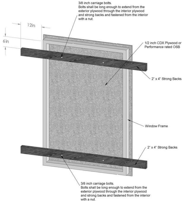
FIGURE 803.1(1) BOARDING OF DOOR OR WINDOW
