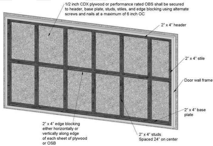
FIGURE 803.1(2) BOARDING OF DOOR WALL
